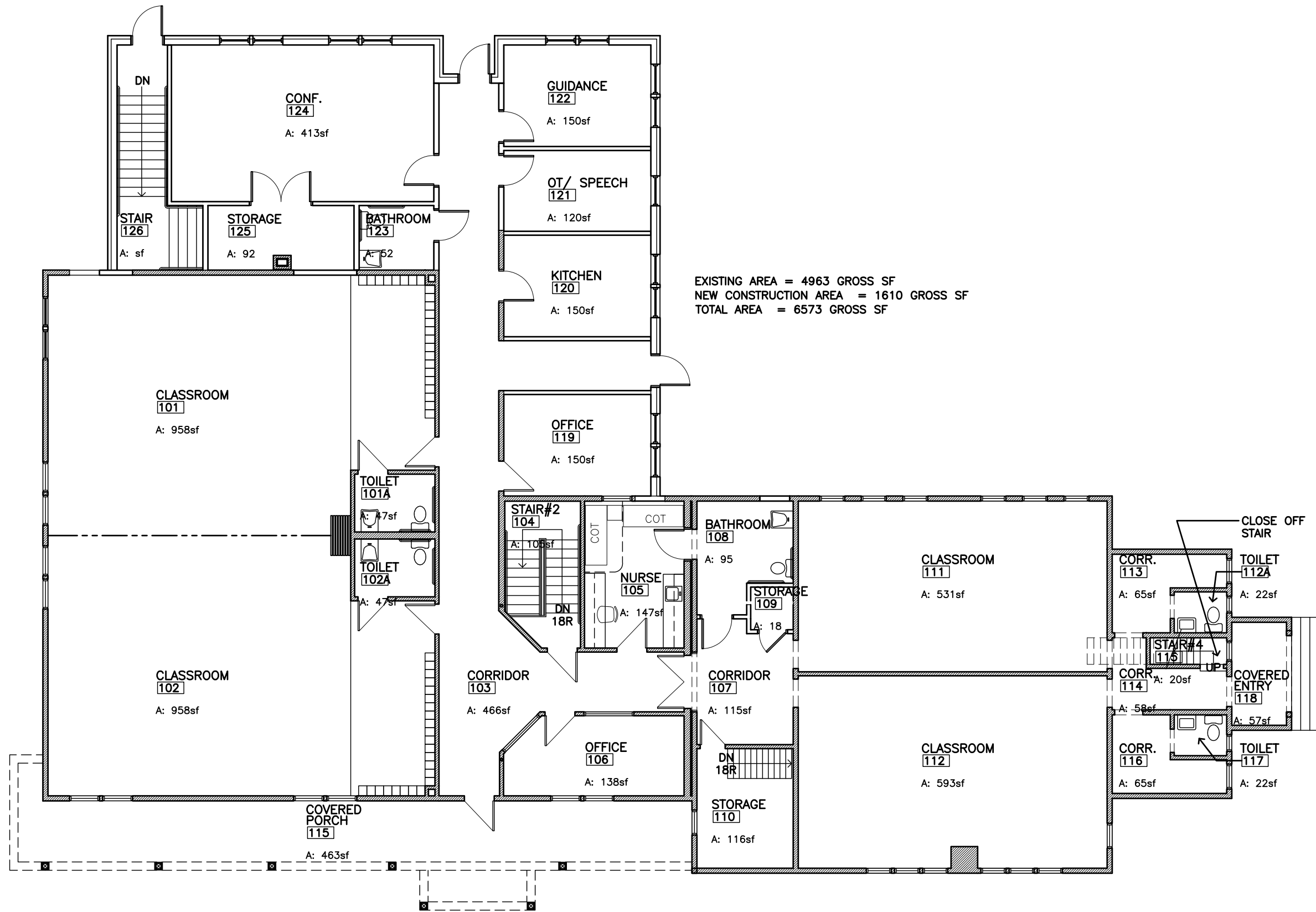
01 FIRST FLOOR PLAN SCALE: 3/32"=1'-0"
